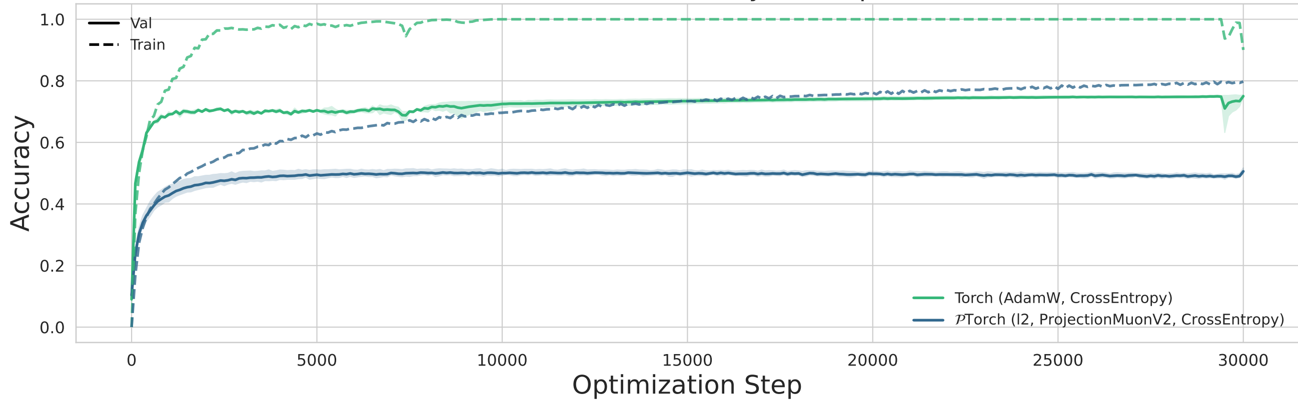
CIFAR10 — Accuracy vs. Step
